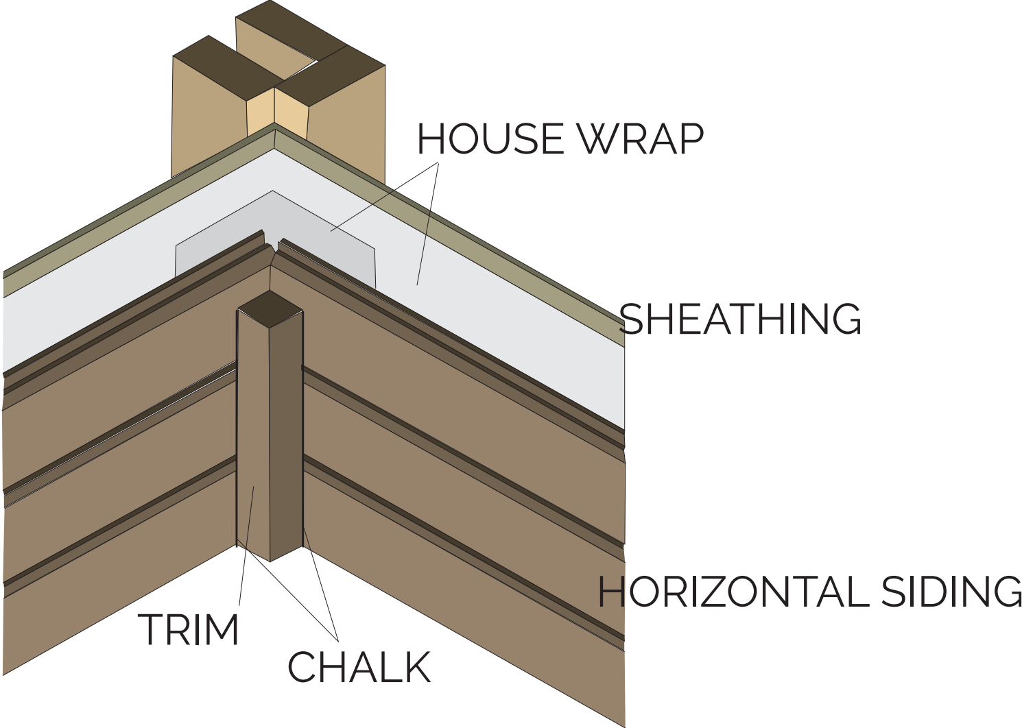
INSIDE CORNER DETAIL-a
